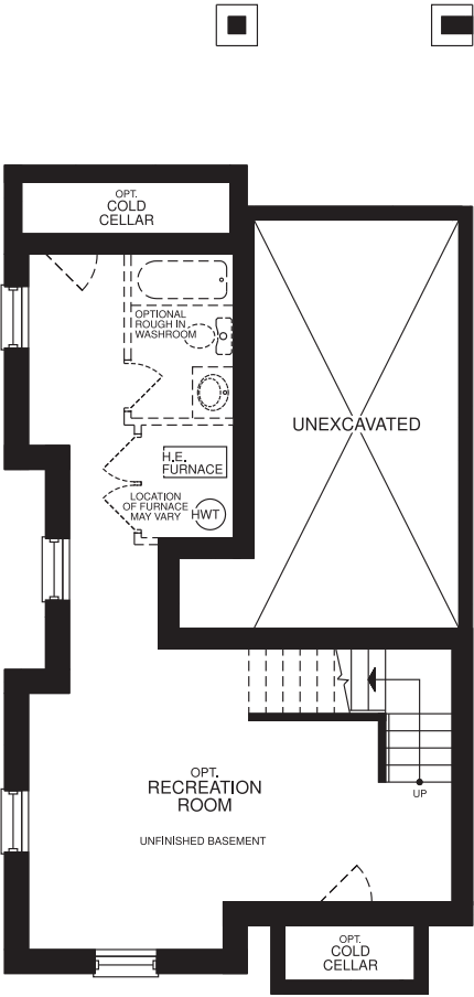
BASEMENT PLAN
