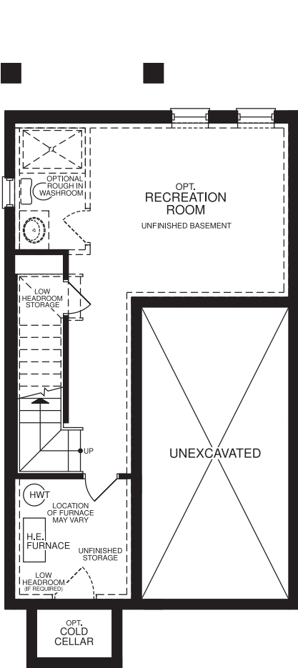
BASEMENT PLAN
