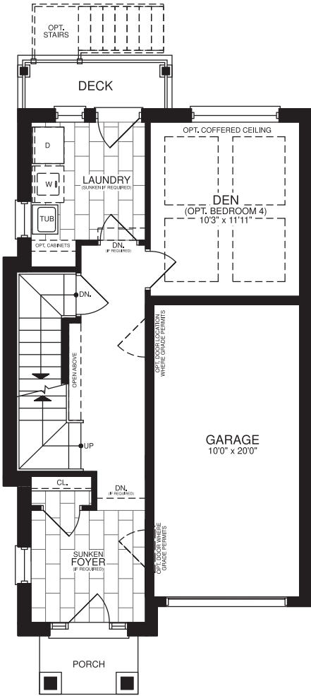
OPT. FIRST FLOOR PLAN WITH DEN
