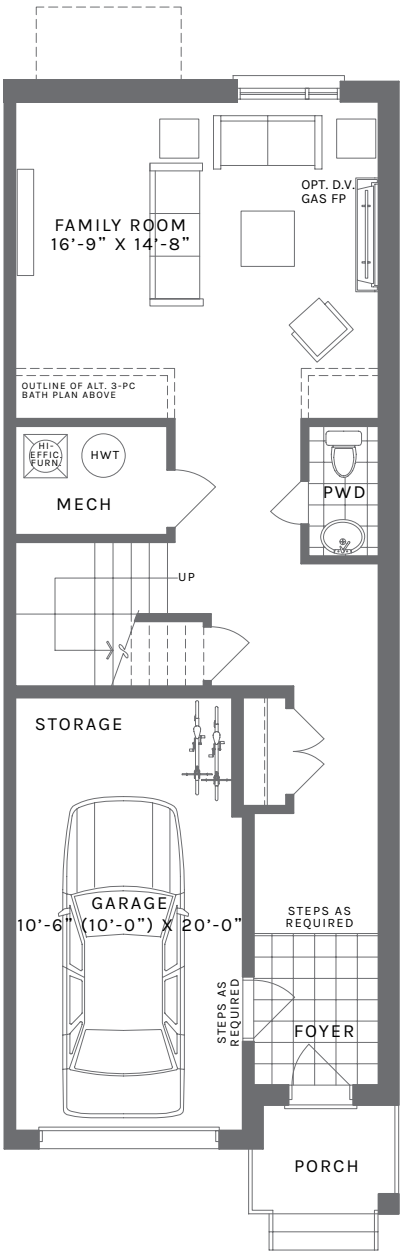
GROUND FLOOR PINE/WALNUT
