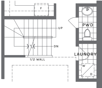
MAIN FL. LAUNDRY FOR ALT. 3-BED PLAN
