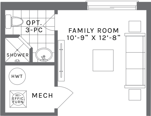
OPTIONAL. 3-PC BATH PLAN
