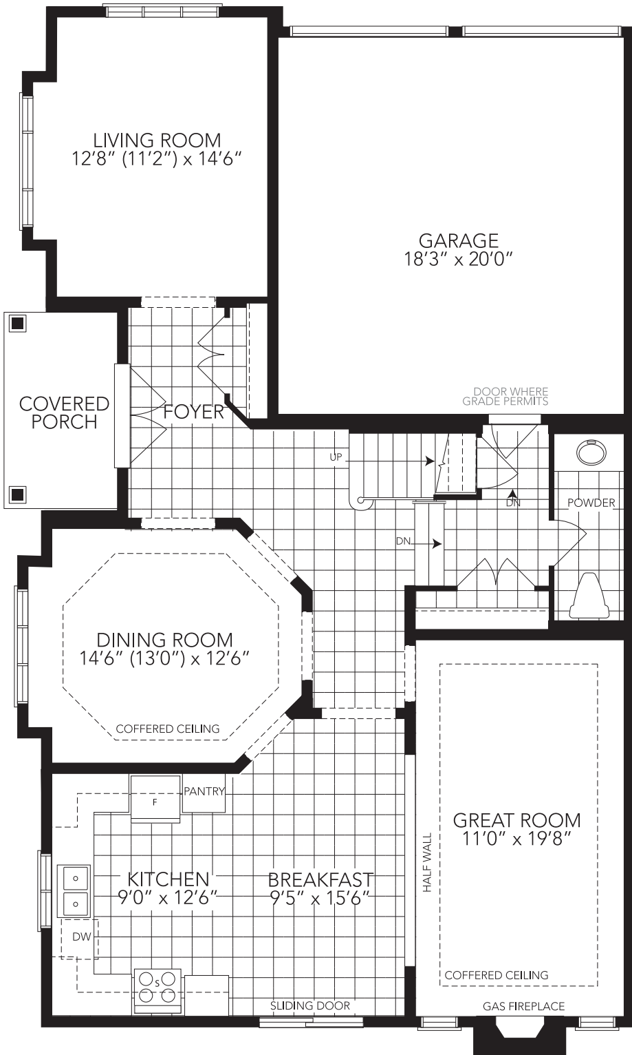
MAIN FLOOR
