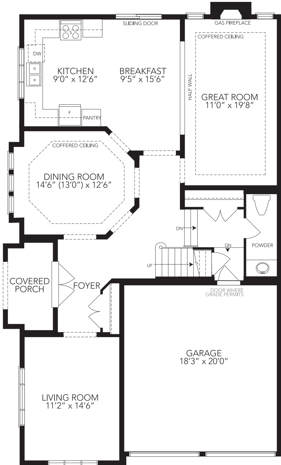
MAIN FLOOR
