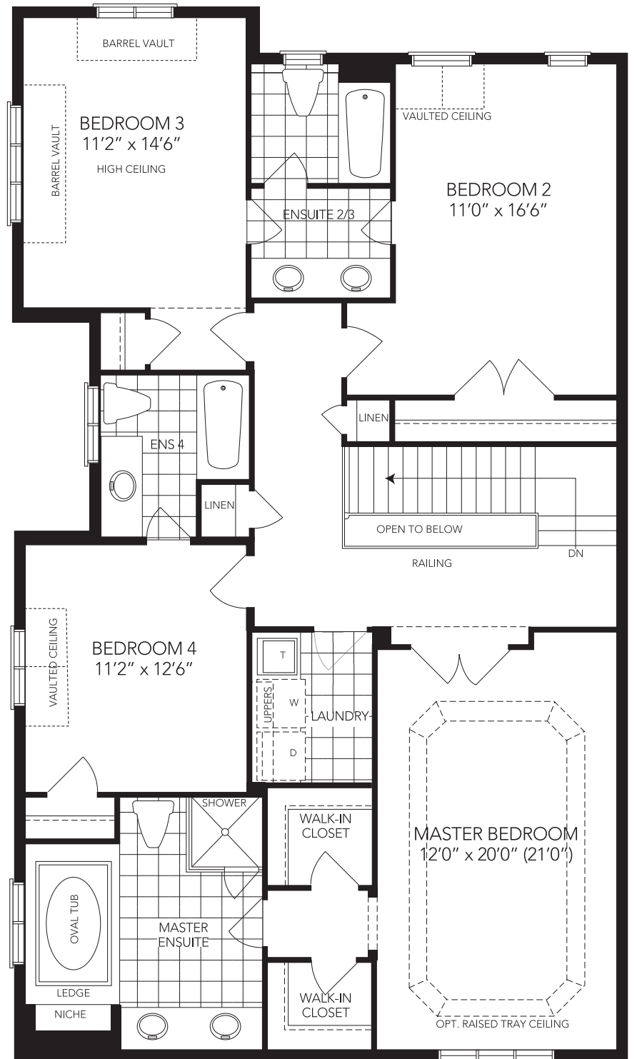
UPPER FLOOR
