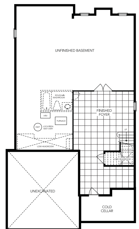
LOWER LEVEL
