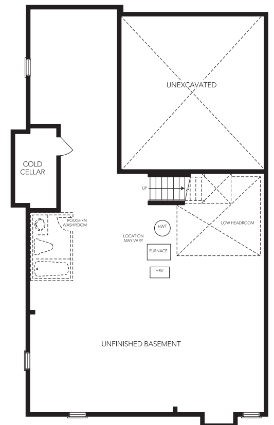
LOWER LEVEL
