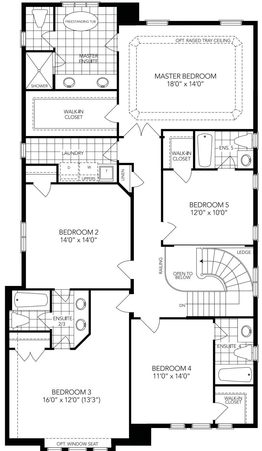
UPPER LEVEL
