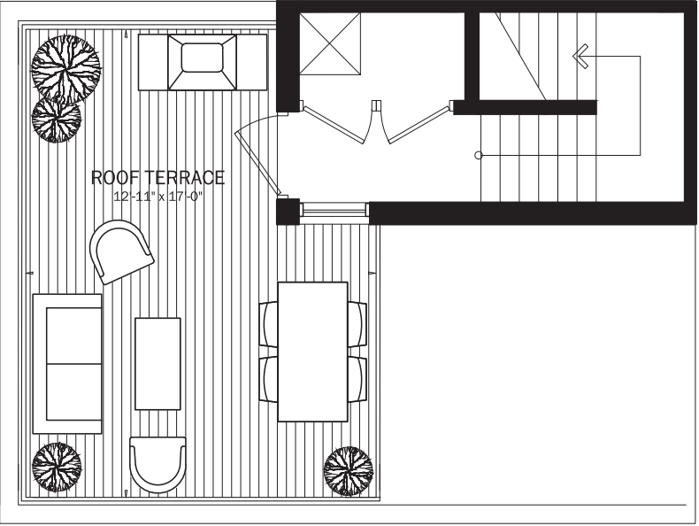
ROOFTOP
