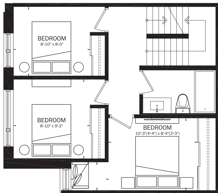
THIRD FLOOR
