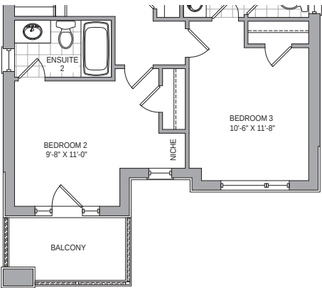
PARTIAL SECOND FLOOR ELEV C2
