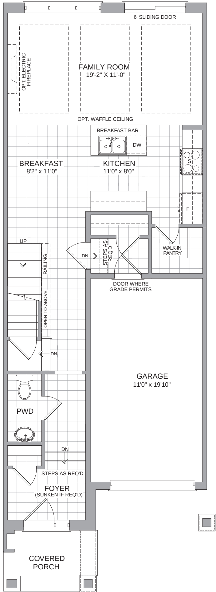
GROUND FLOOR ELEV C1
