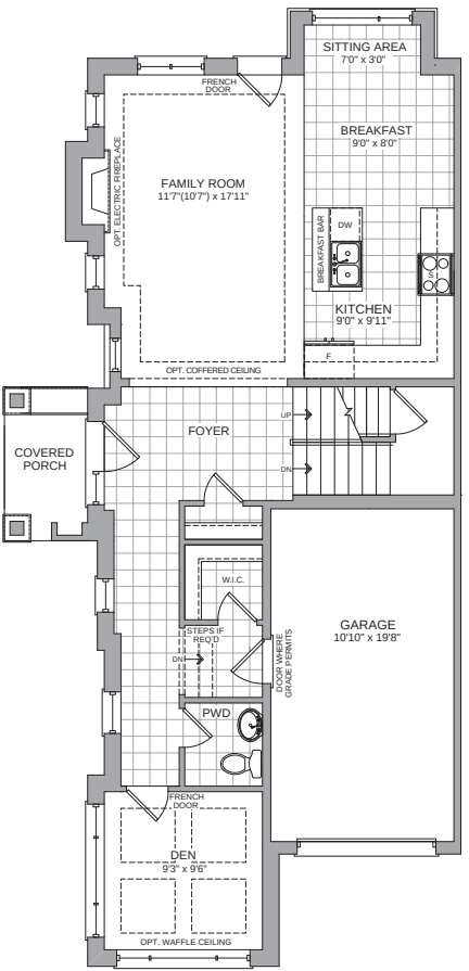
GROUND FLOOR ELEV C2
