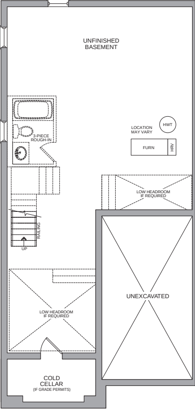
BASEMENT ELEV C1 LEFT + RIGHT
