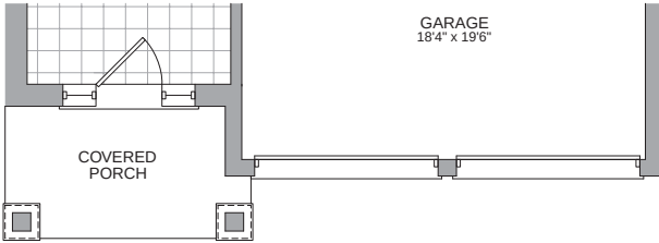
PARTIAL GROUND FLOOR ELEV C2
