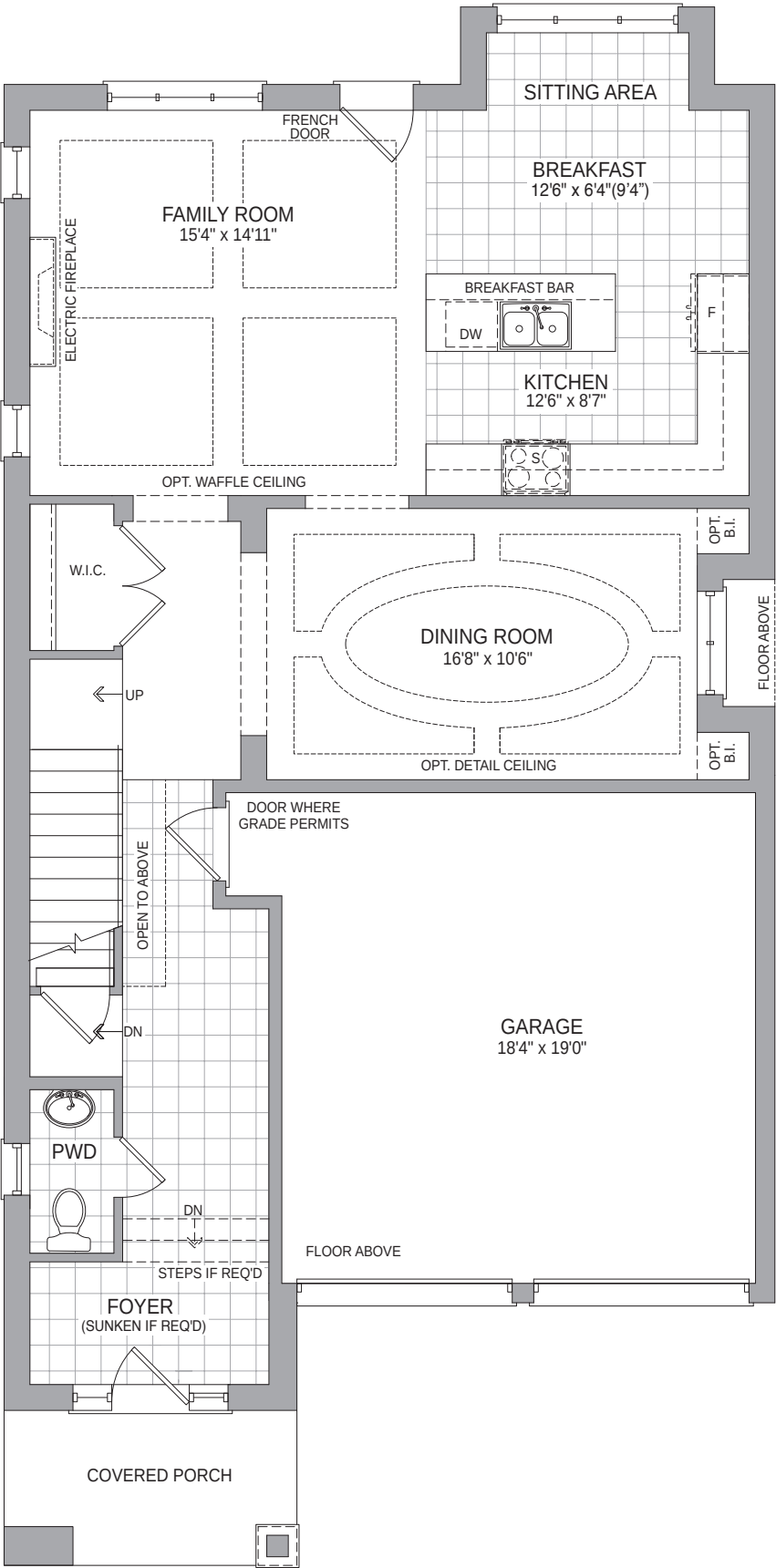
GROUND FLOOR ELEV C1
