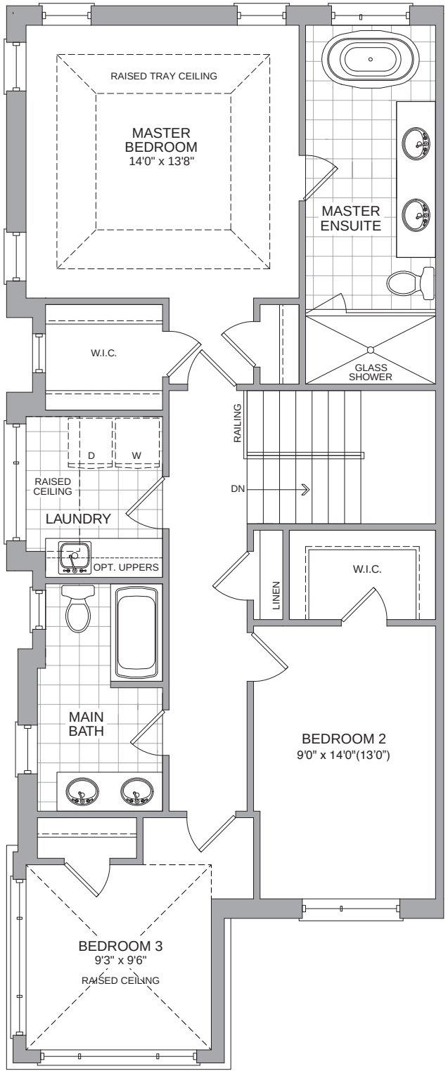
SECOND FLOOR ELEV C1
