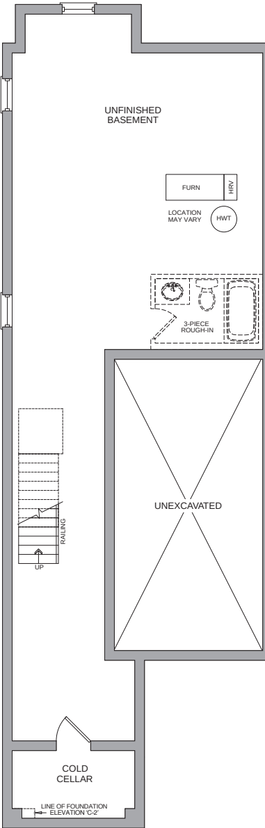
BASEMENT ELEV C1 & C2
