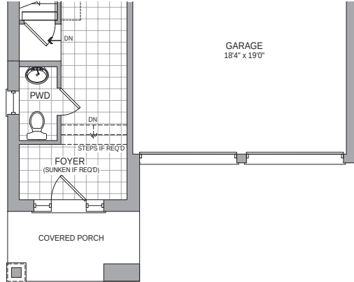
PARTIAL SECOND FLOOR ELEV C2
