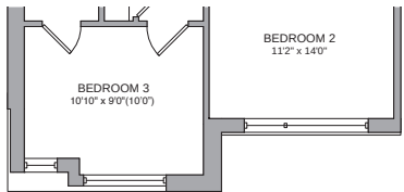
SECOND FLOOR ELEV C2 LEFT
