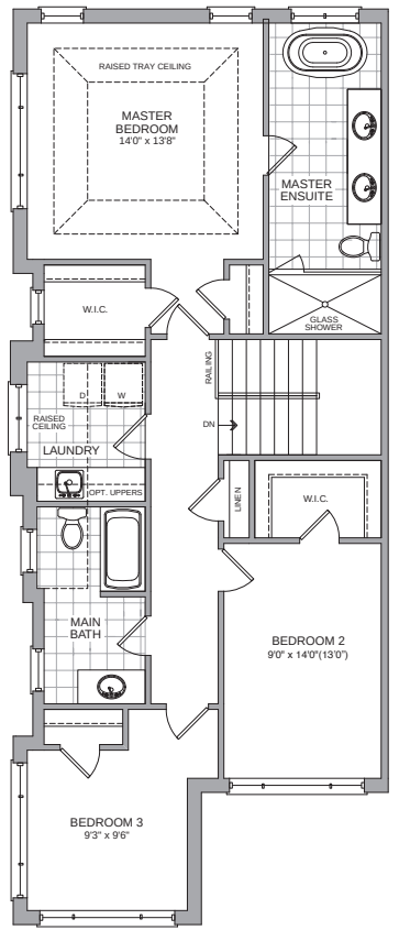
SECOND FLOOR ELEV C2
