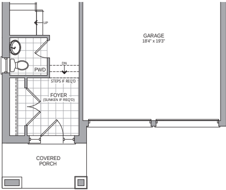
PARTIAL GROUND FLOOR ELEV C2
