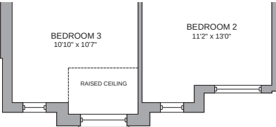
SECOND FLOOR ELEV C2 LEFT + RIGHT
