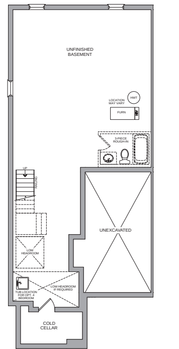
BASEMENT ELEV C1 LEFT + RIGHT
