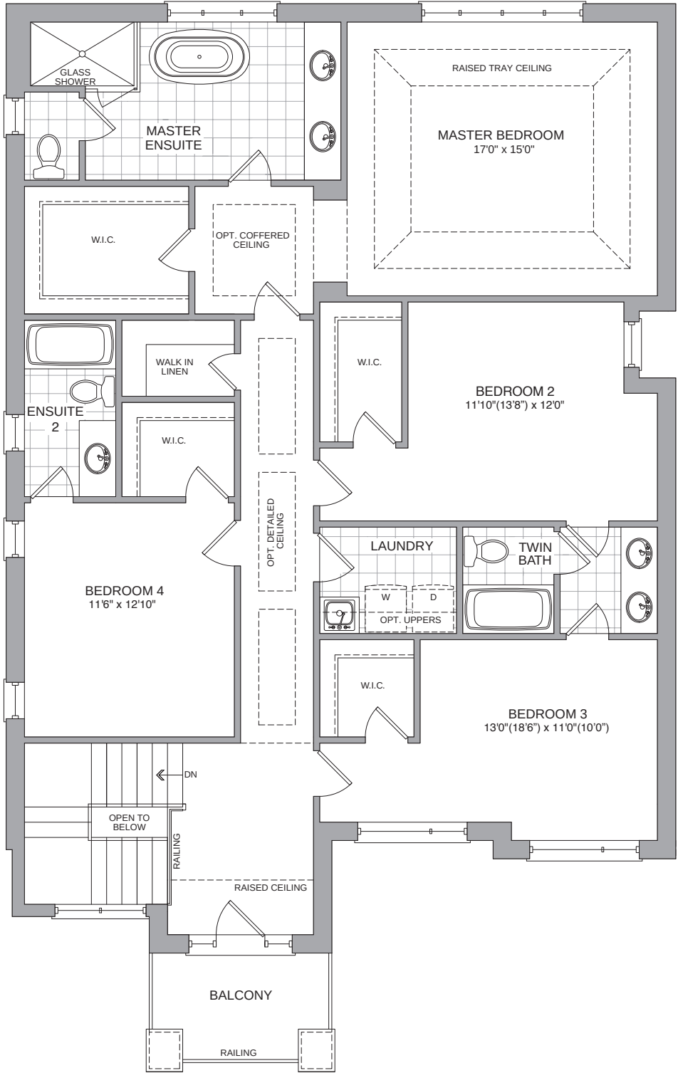
SECOND FLOOR ELEV C1
