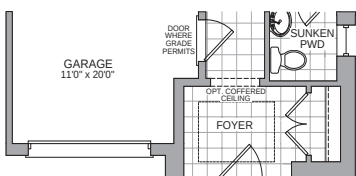
PARTIAL GROUND FLOOR ELEV C2 LEFT
