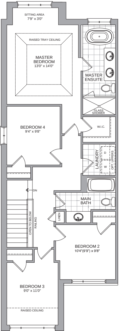
SECOND FLOOR ELEV C1 OPT. 4 BEDROOM
