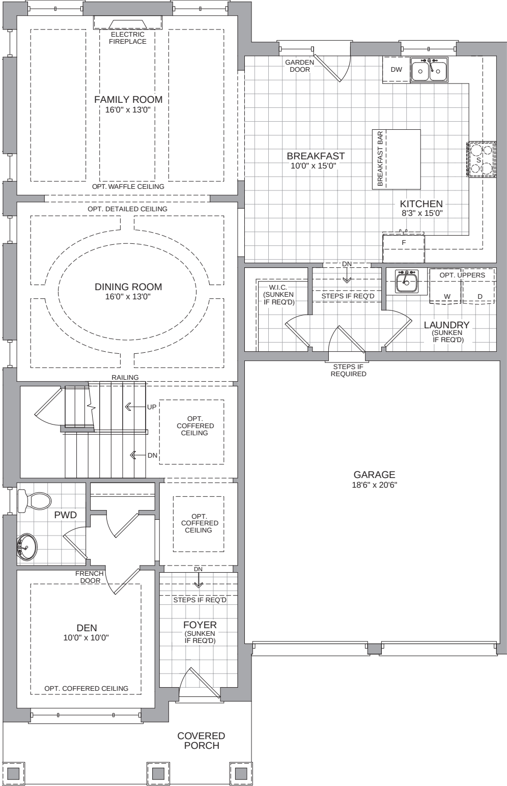
GROUND FLOOR ELEV C1
