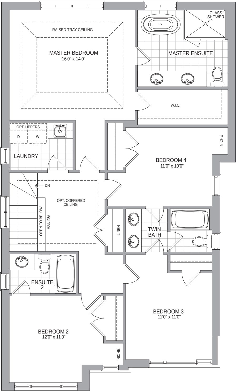
SECOND FLOOR ELEV C1
