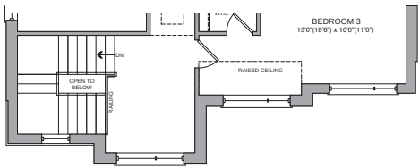
PARTIAL SECOND FLOOR ELEV C2
