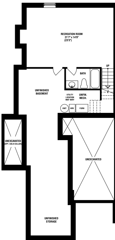
OPT. FIN. BASEMENT PLAN ELEVATION 'A-1', 'B-1' & 'C-1'
