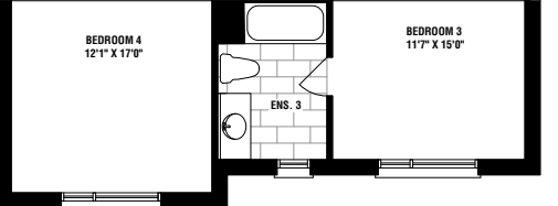
OPT. UPPER FLOOR PLAN ELEV. 'C'
