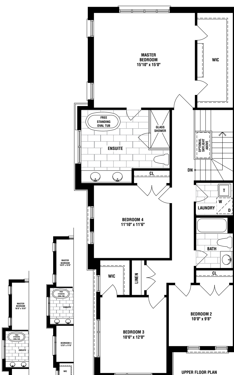
UPPER FLOOR PLAN ELEVATION 'A-1'
