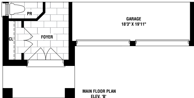
MAIN FLOOR PLAN ELEV. 'B'
