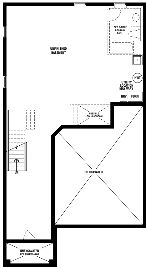
BASEMENT PLAN ELEV. 'A'
