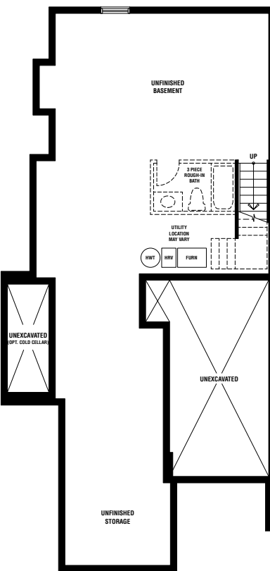
BASEMENT PLAN ELEVATION 'A-1', 'B-1' & 'C-1'
