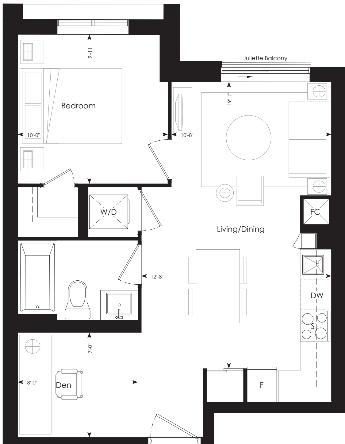
15TH-35TH FLOORPLAN
