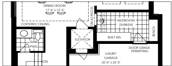
PART. GROUND FLOOR WITH ELEVATOR ELEVATION A & B
