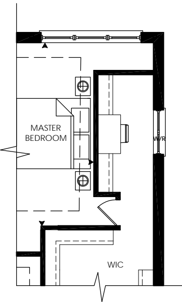
SECOND LEVEL WITH OPT. WARDROBE PLAN
