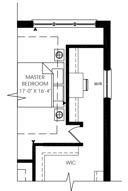
SECOND LEVEL WITH OPT. WARDROBE PLAN
