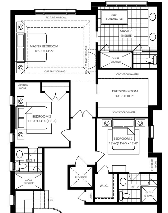
PART. OPTIONAL SECOND FLOOR WITH ELEVATOR ELEVATION A & B
