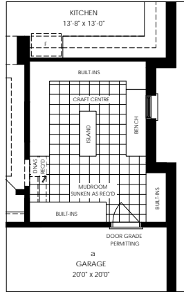
OPTIONAL GROUND FLOOR WITH CRAFT ROOM
