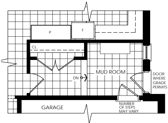
GROUND LEVEL WITH OPT. MUD ROOM PLAN
